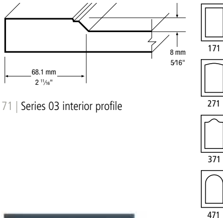
Model 3171 Regular rails
